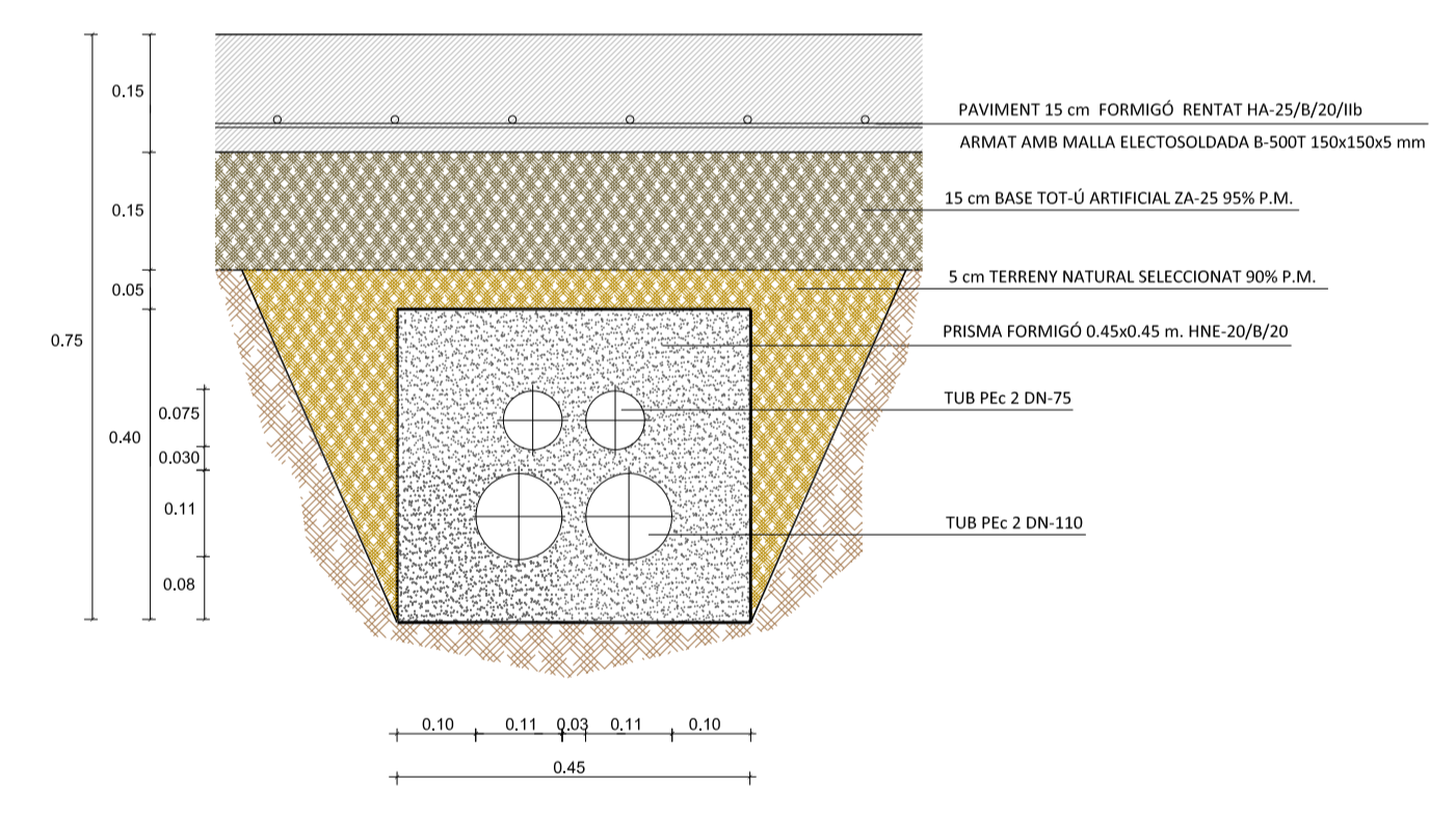
DETALL RASA TUB PEc 2 DN 110 + 2 DN 75 E= 1/10
