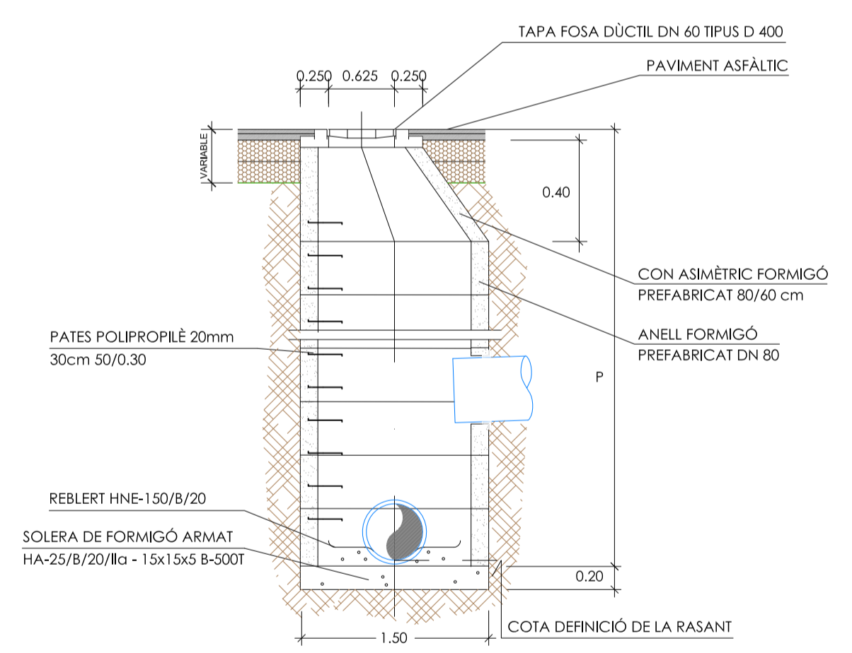
DETALL POU RASANTS E= 1/50
