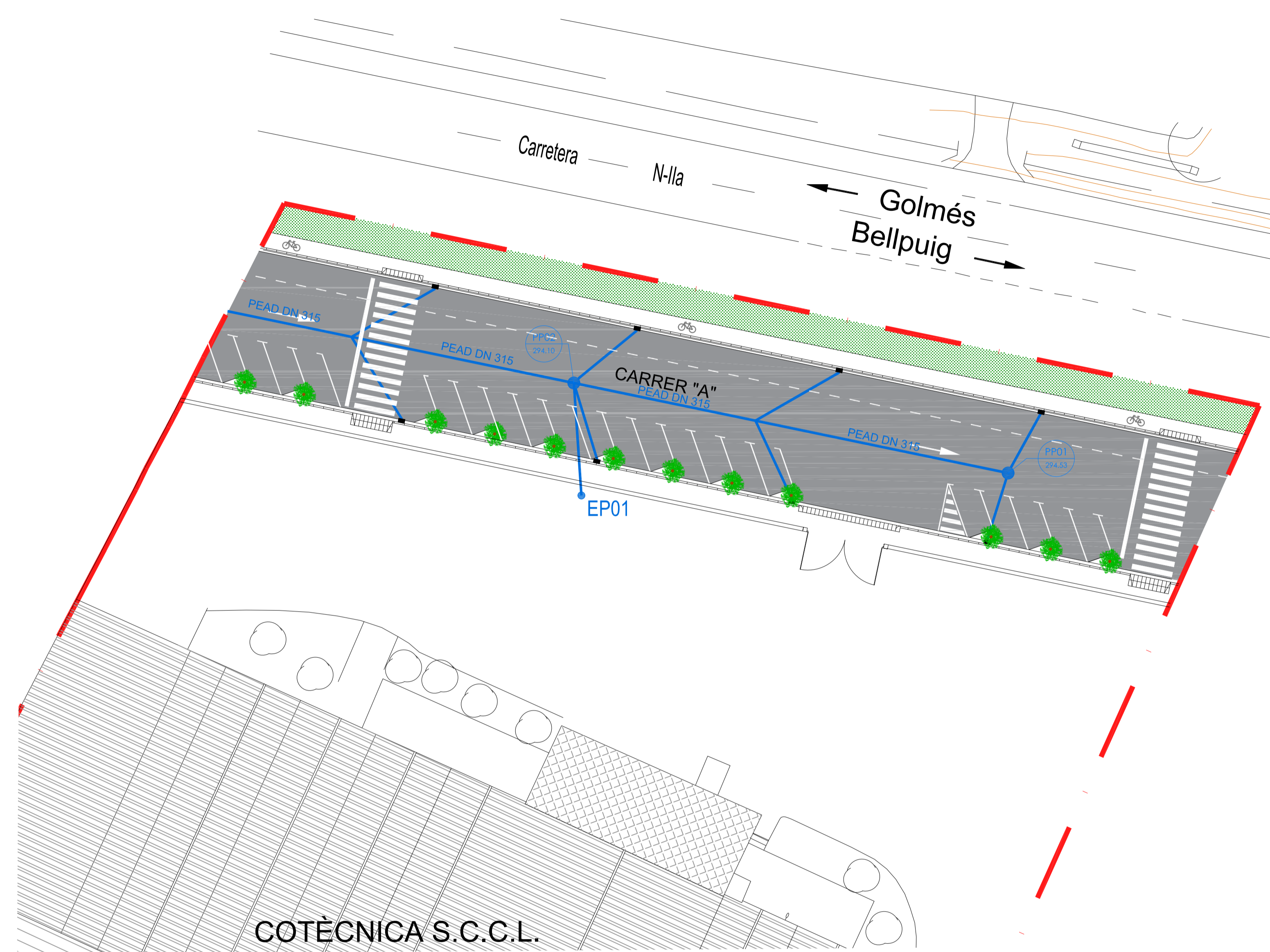
PLANTA GENERAL E= 1/300
